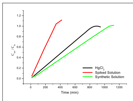
Fig. 8. Breakthrough curve
