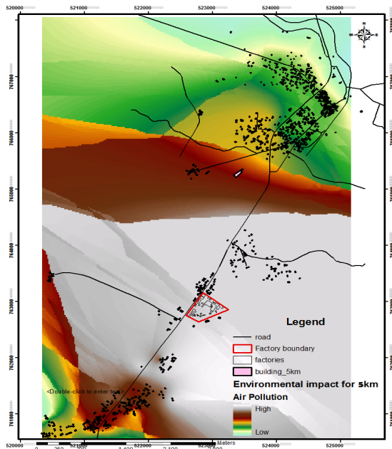
Fig. 10 Map showing the Level of Air pollution
