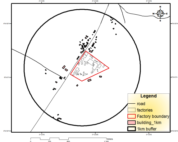
Fig. 7 Ewekoro Cement Factory Environs within 1km
