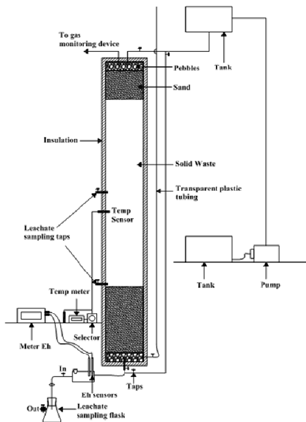
Fig. 1 Reactor assembly
