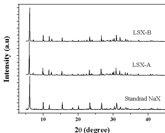
Fig. 1 XRD spectrum of zeolite LSX-A, LSX-B and standard NaX
