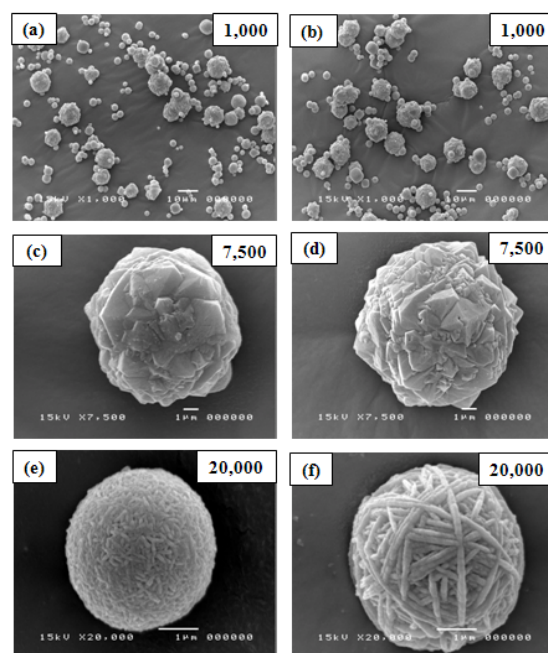
Fig. 2 SEM images of zeolite LSX-A and LSX-B at different magnification
