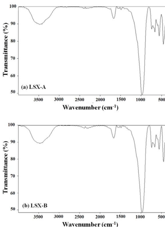
Fig. 3 The FTIR spectra of zeolite LSX-A and LSX-B
