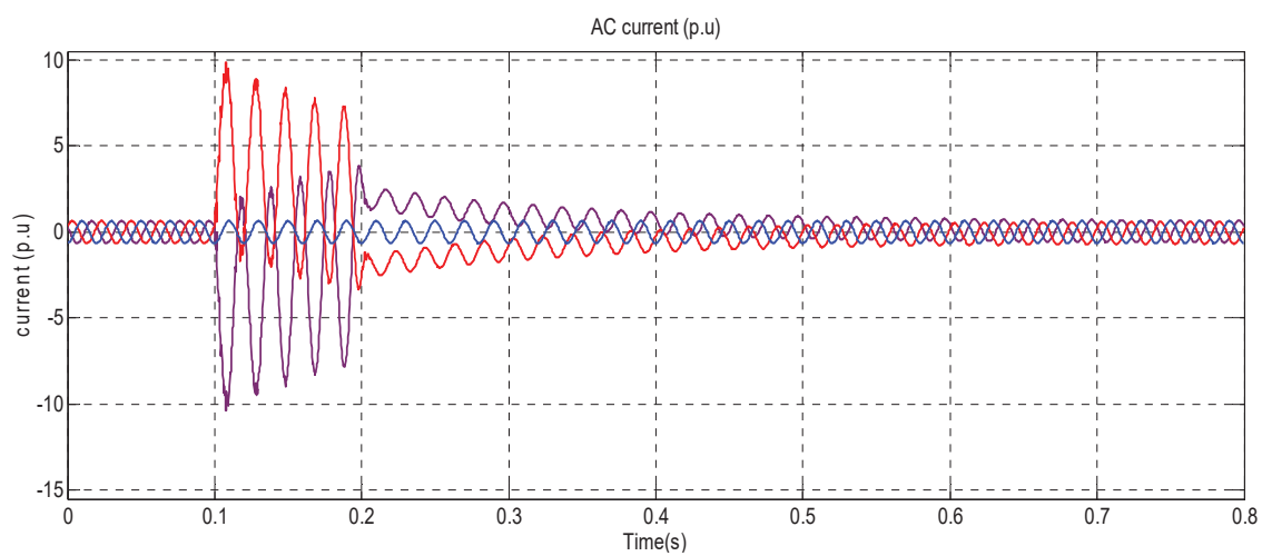
Fig. 6 HVAC Line Fault current at B2
