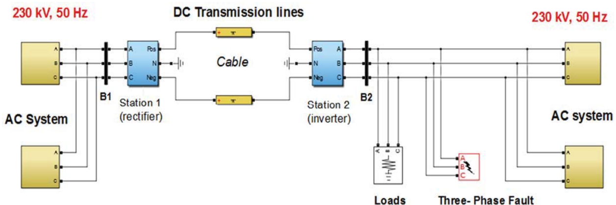
Fig. 3 HVDC Power Transmission System
