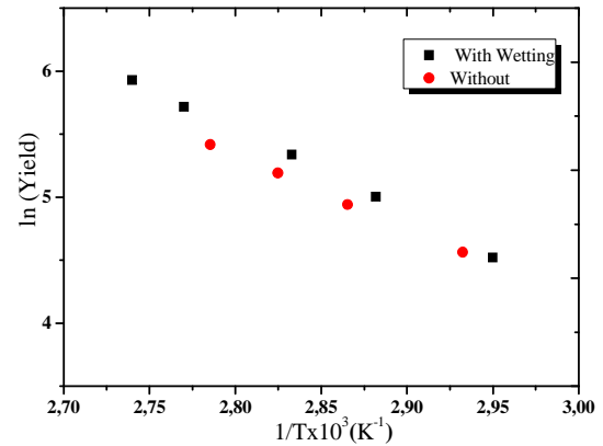
Fig. 4 Effects of tray surface wetting on Yield
