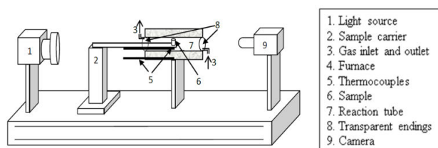
Fig. 5 Typical heating microscope
