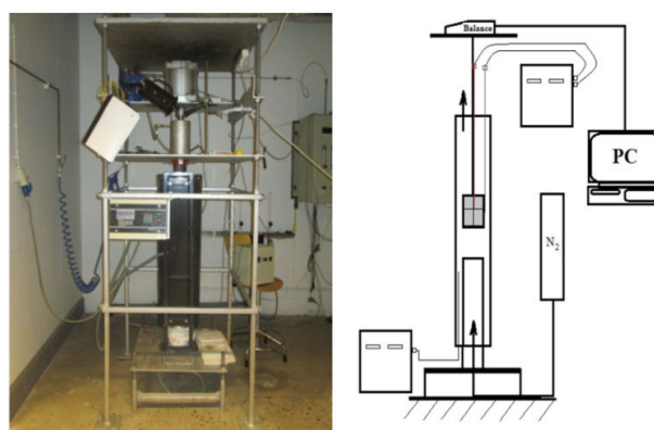
Fig. 3 Photo image and schematic diagram of the furnace assembly
