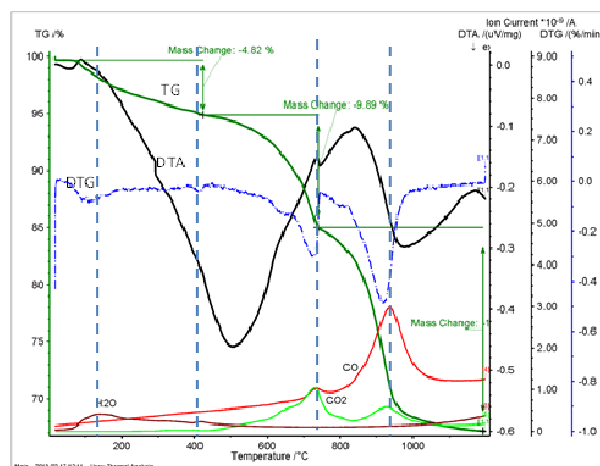
Fig. 7 Thermal analysis curves of BM1 as a function of Temperature
