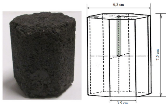
Fig. 1 Photo image as well as schematic diagram of used briquettes
