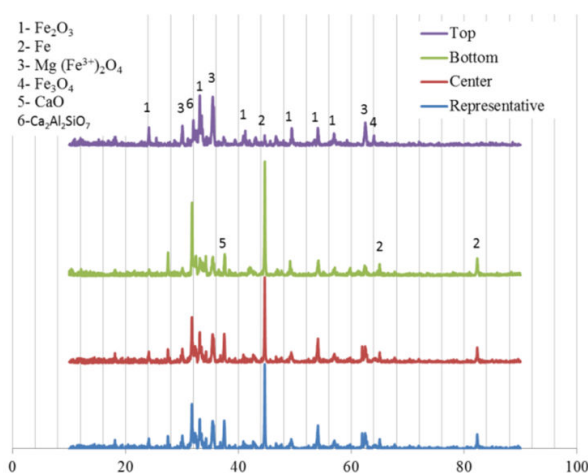
Fig. 12 XRD of reduced briquette (B1)
