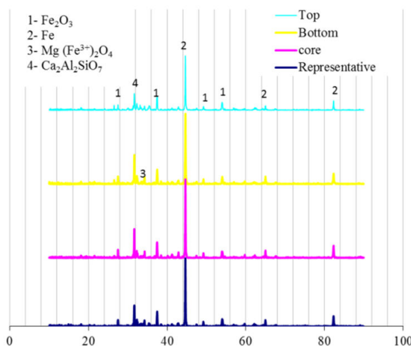
Fig. 13 XRD of reduced briquette (B4)
