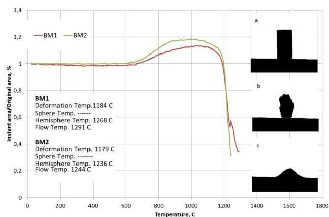
Fig. 11 Selected images show the sample deformation and melting (on the right hand side) and the change of sample silhouette area as a function of temperature (On the left hand side)
