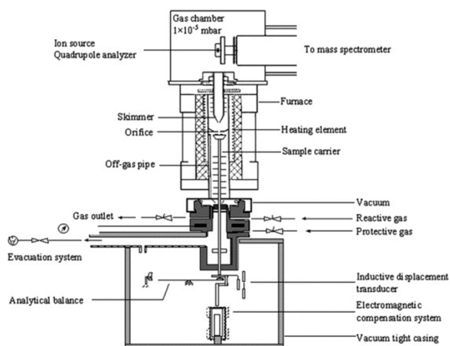
Fig. 2 Illustration of TGA/DTA/QMS
