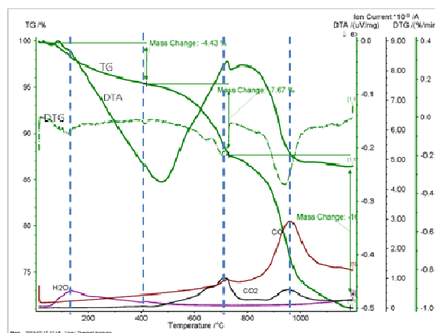
Fig. 8 Thermal analysis curves of BM2 as a function of Temperature
