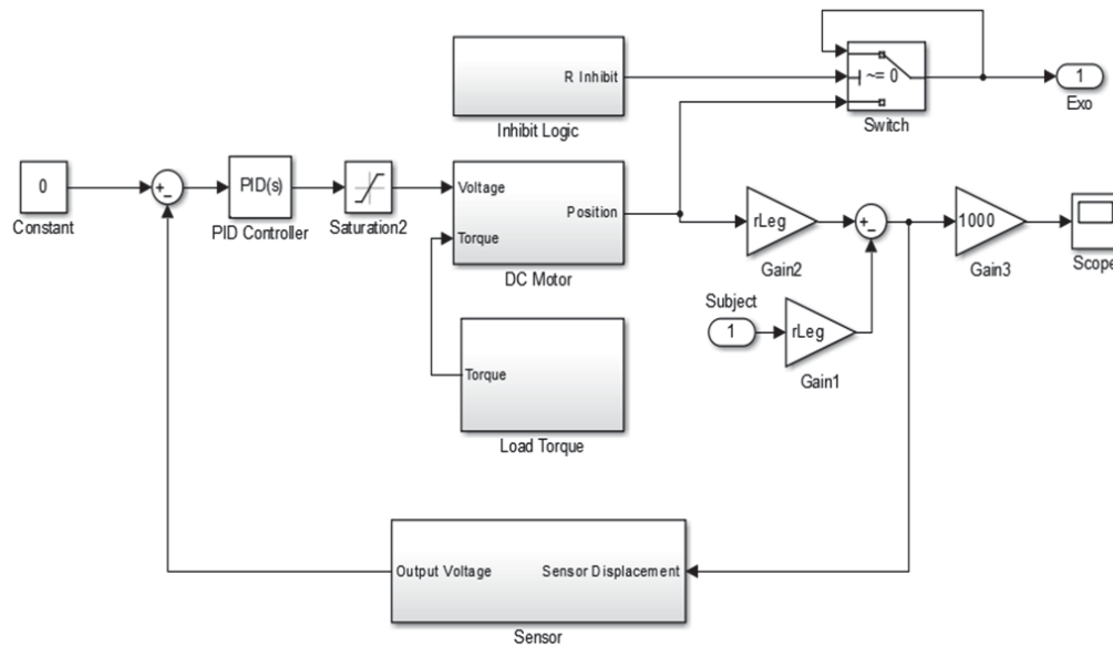
Fig. 7 Closed-loop controller for knee joint
