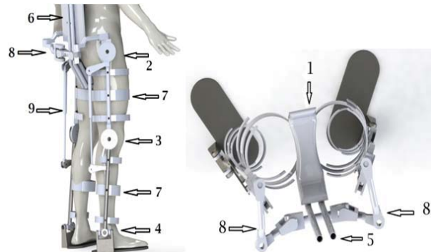
Fig. 1 Components of the exoskeleton
