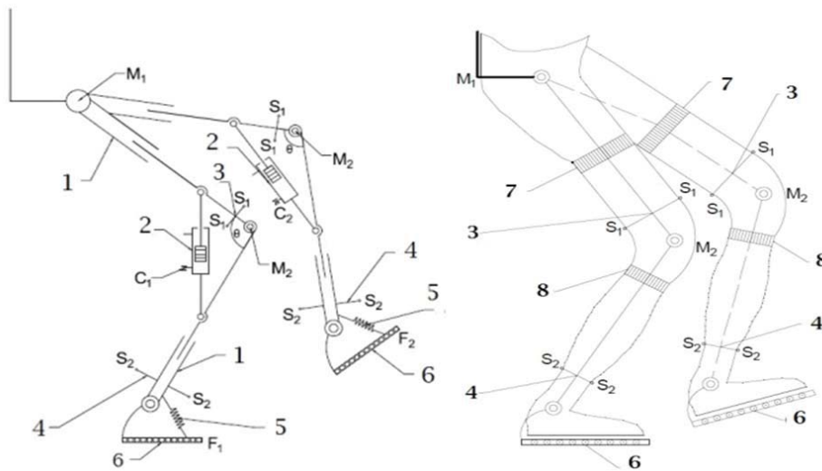
Fig. 2 Schematic drawing of the exoskeleton
