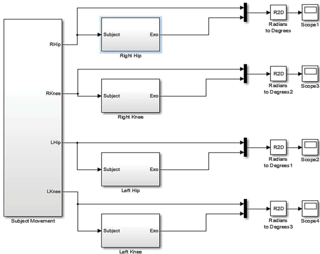
Fig. 5 Top layer of exoskeleton simulation program
