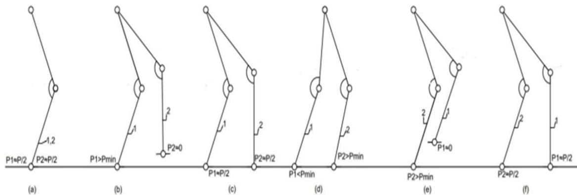
Fig. 3 Gaits of the exoskeleton
