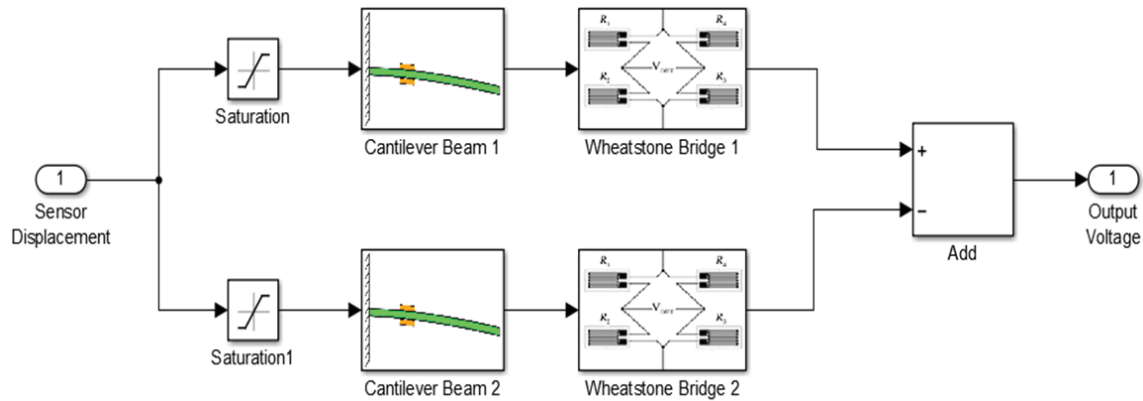
Fig. 8 Simulink model of the sensing subsystem
