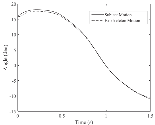
Fig. 9 Hip joint angle during leg swinging motion
