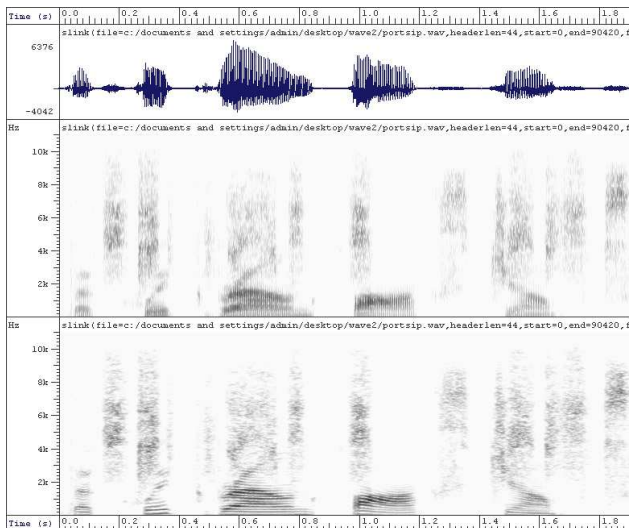
Fig. 7 PortSIP Waveform, Wideband and Narrowband spectrograms
