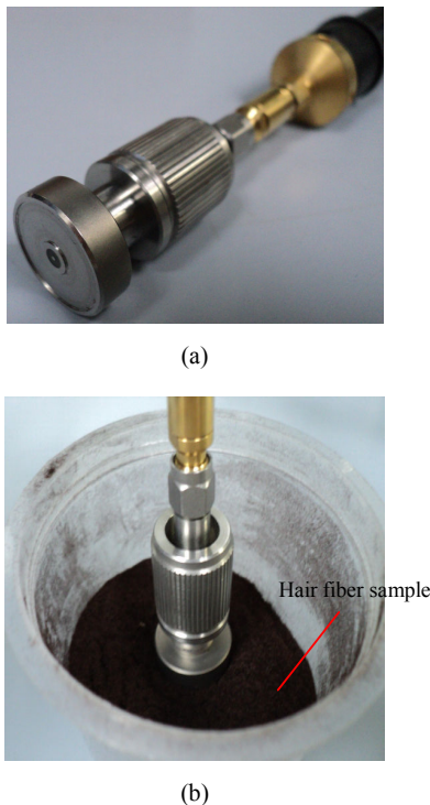
Fig. 12 (a) Keysight 85070D dielectric probe (b) Hair fiber dielectric measurement using 85070D dielectric probe
