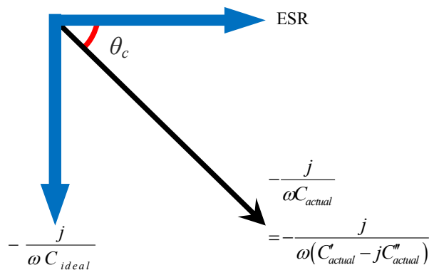
Fig. 7 Vector diagram of the impedance, Z
