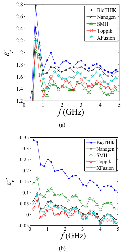
Fig. 13 The measured (a) \epsilon_r' and (b) \epsilon_r'' of the five types of hair fibers using 85070D dielectric probe
