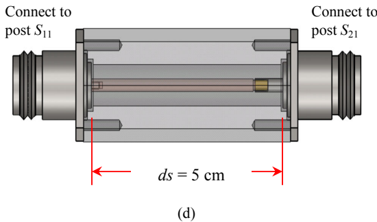
Fig. 9 (a) Components of coaxial waveguide (b) Fully-filled hair sample in coaxial line (c) Experimental setup (d) Dimension of coaxial waveguide
