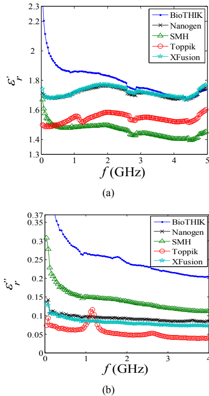
Fig. 11 The calculated (a) \epsilon_r' and (b) \epsilon_r'' of the five types of hair fibers
