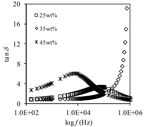
Fig. 4 Variation of \tan \delta with frequency for selected samples
