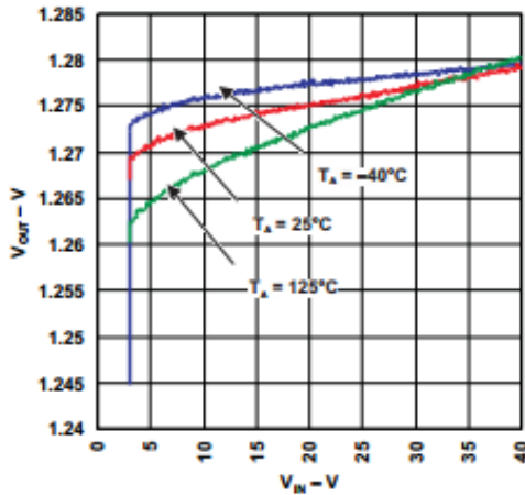
Fig. 8 Line regulation
