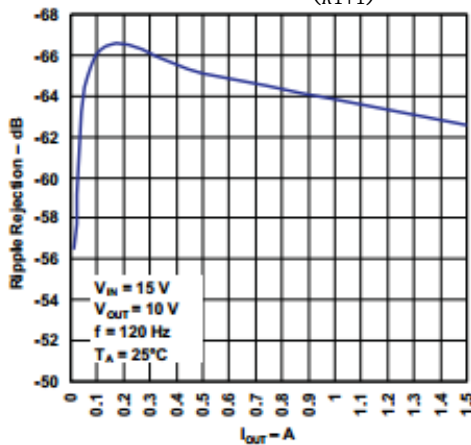
Fig. 9 Ripple rejection
