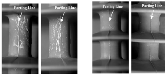
(a) Straight Shed (b) Alternate Shed Fig. 4 Ageing of specimen surface after 50 Test Cycles
