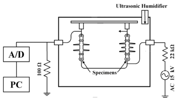
Fig. 2 Test Arrangement
