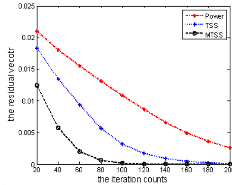
Fig. 2. Graph for an intuitive comparison of the numerical results in Table 1.
