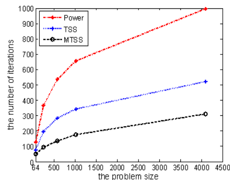
Fig. 3. Comparisons of the iteration counts for the Power, TSS and MTSS iteration methods with the different sized tandem queueing networks.
