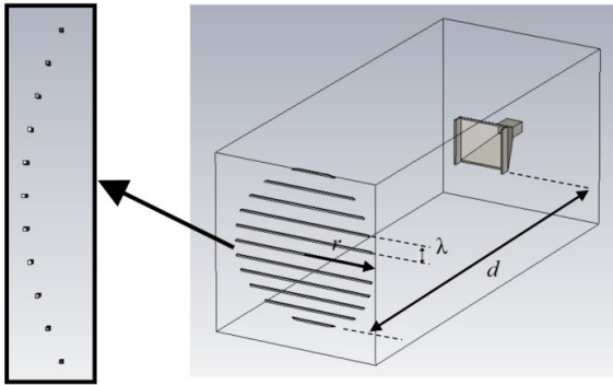
Fig. 4 A rectangular horn antenna with two wing slabs and various shaped woodpile EBG
