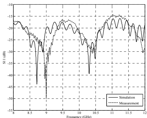
Fig. 11 The reflection coefficient of the proposed antenna
