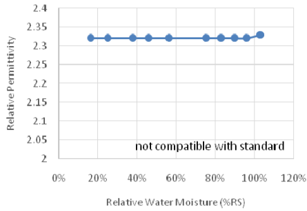
Fig. 8 Dependence of Relative Permittivity on Water content
