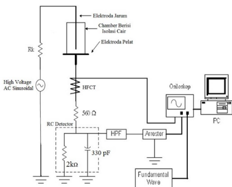
Fig. 5 Schematic circuit for PD measurement
