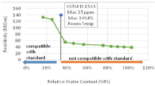
Fig. 9 Dependence of resistivity on water content
