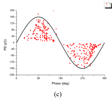
Fig. 14 \phi - q - n PD patterns of Sample (a) M03 (b) M05 and (c) M10 at applied voltage of 11 kV
