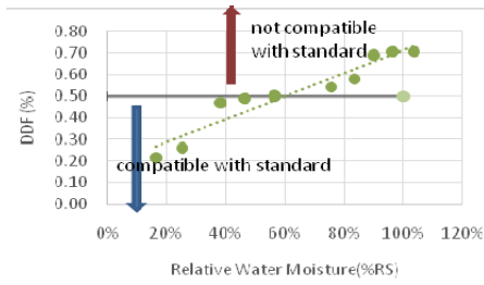
Fig. 7 Dependence of Dissipation Factor on Water content
