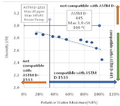
Fig. 10 Dependence of viscosity on water content
