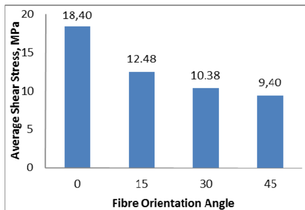
Fig. 3 Shear stresses of the adhesive, Hysol EA 9394, against fiber orientation angle of the composite adherents
