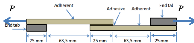
Fig. 2 Single lap joint specimens for shear performance of the adhesive under tensile loading
