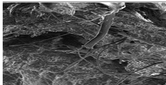
Fig. 7 Morphology of 1 weight % of silane loading into HDPE/Henequen microfiber compositions at 3000 x magnification
