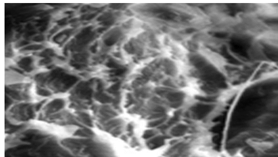
Fig. 6 Morphology of 0.9 weight% of silane loading into HDPE/Henequen microfiber compositions at 3000 x magnification
