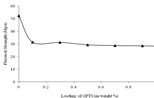
Fig. 1 Variation in flexural strength of HDPE/Henequen microfibrer (8 weight %) composite with silane weight % loading
