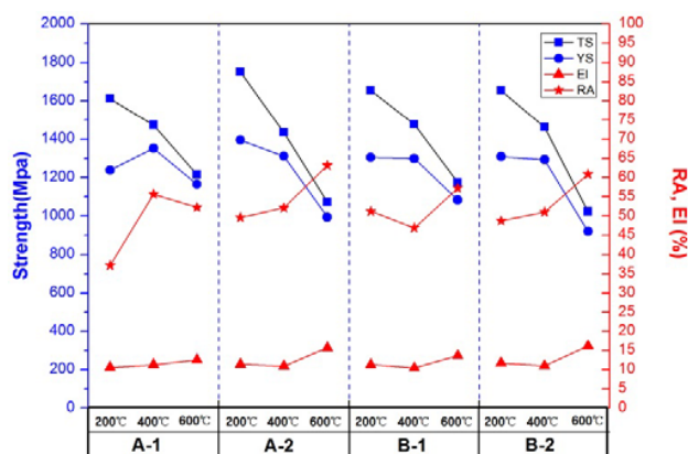
Fig. 2 Variation of the mechanical properties according to tempering temperature
