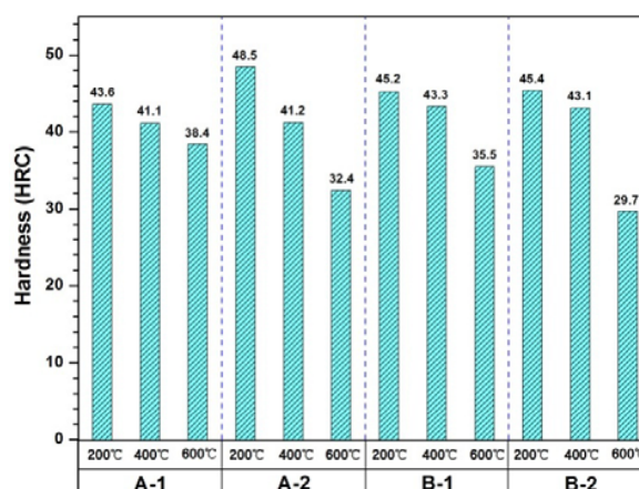
Fig. 3 Variation of the hardness with different tempering temperatures
