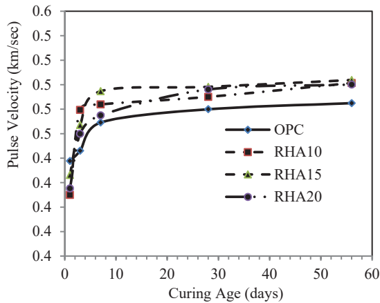
Fig. 7 Ultrasonic Pulse Velocity of HSHPC
