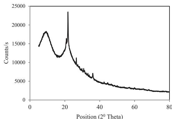
Fig. 2 The XRD of RHA
