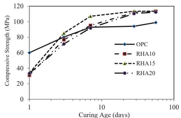
Fig. 3 Compressive Strength of HSHPC
