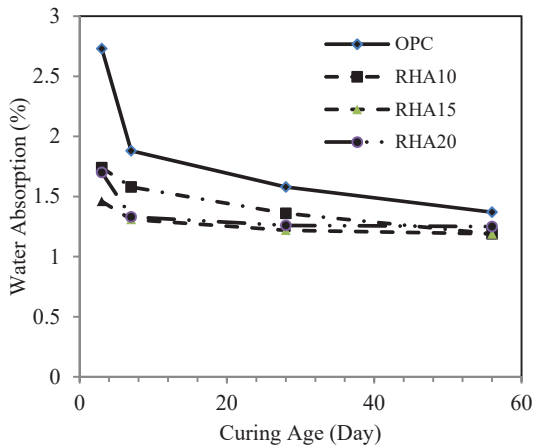
Fig. 4 Water Absorption of HSHPC
