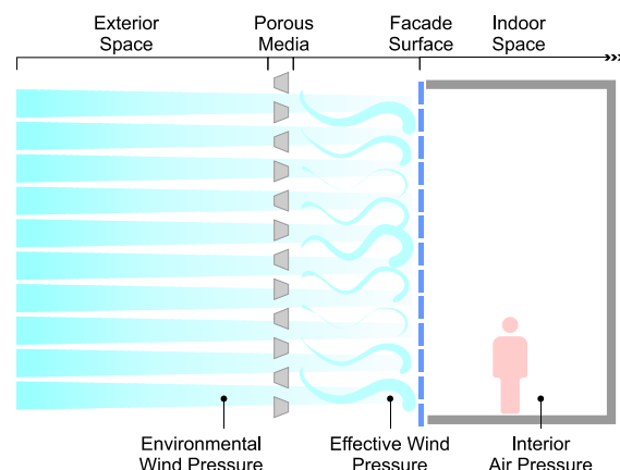
Fig. 3 Diagram of Porous Façade under Low Wind Speed
