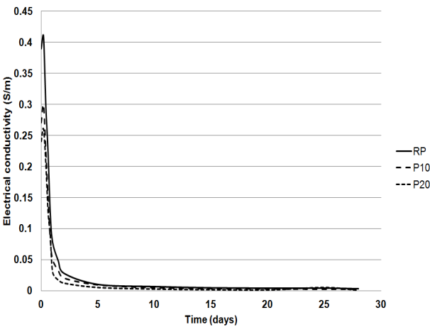
Fig. 4 Electrical conductivity of studied pastes measured for time interval of 28 days
