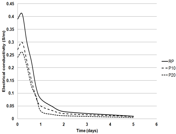
Fig. 3 Changes of electrical conductivity of studied pastes within first 5 days from casting
