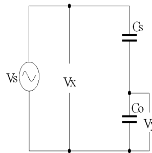
(a) Sawyer-Tower circuit diagram ( C_0=1\mu\text{F} , C_s= sample; C_0 \gg C_s )
