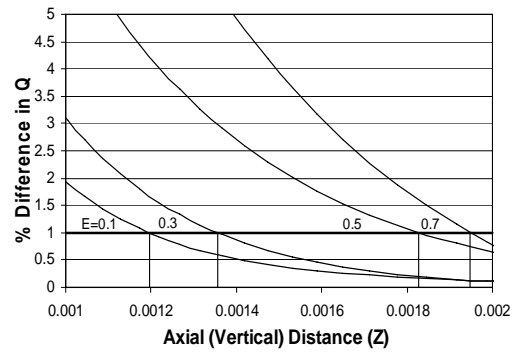
Fig. 7 Annulus axial heights required for thermal full development at different values of eccentricity
