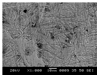
Fig. 3 (d) Microstructure of sample austenitized at 975^{\circ}\text{C} and austempered at 325^{\circ}\text{C} for 6 hours
