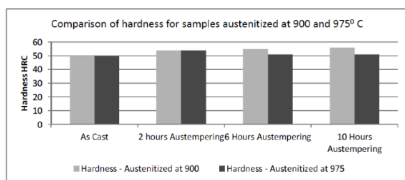
Fig. 4 Hardness comparison
