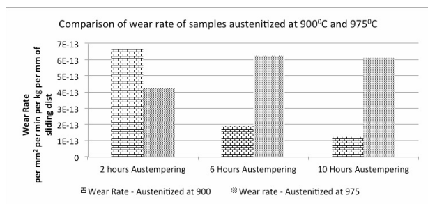
Fig. 5 Wear rate comparison
