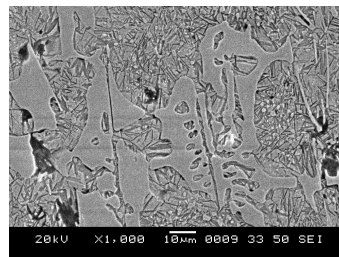
Fig. 3 (b) Microstructure of sample austenitized at 975^{\circ}\text{C} and austempered at 325^{\circ}\text{C} for 2 hours
