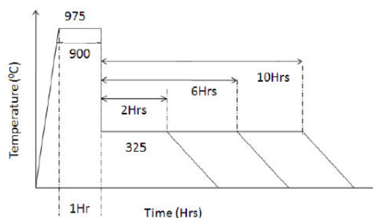
Fig. 1 Schematic representation of austempering treatment employed
