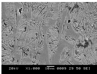
Fig. 3 (f) Microstructure of sample austenitized at 975 o C and austempered at 325 o C for 10 hours
