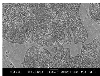
Fig. 3 (e) Microstructure of sample austenitized at 900^{\circ}\text{C} and austempered at 325^{\circ}\text{C} for 10 hours
