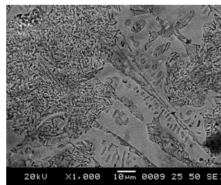
Fig. 3 (a) Microstructure of sample austenitized at 900^{\circ}\text{C} and austempered at 325^{\circ}\text{C} for 2 hours
