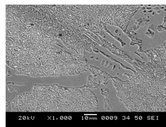
Fig. 3 (c) Microstructure of sample austenitized at 900^{\circ}\text{C} and austempered at 325^{\circ}\text{C} for 6 hours
