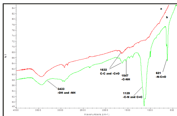
Fig. 1 FTIR spectra of a) pristine carbon nanotube b) amine functionalized carbon nanotube
