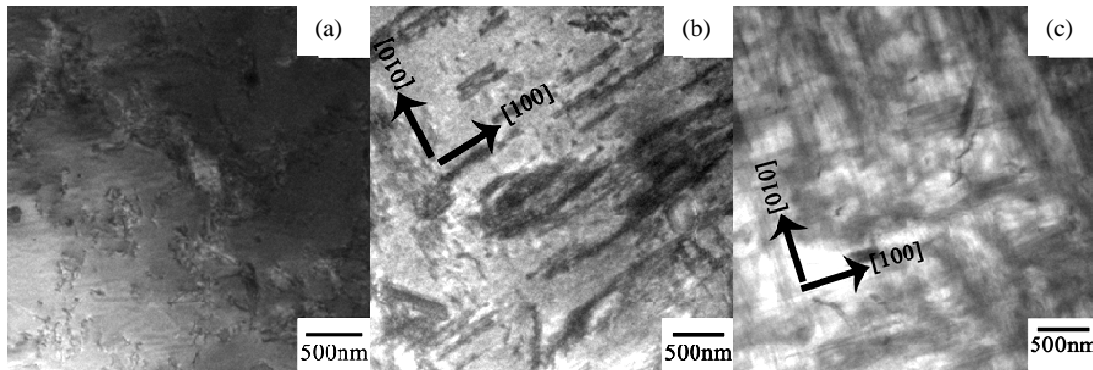
Fig. 2TEM micrographs and SAD patterns at \langle 100 \rangle_{Al} beam direction of the specimens aged at 225 °C for various times of: (a) 15min (underaging), (b) 1h (peak aging), and (c) 12h (overaging), respectively
