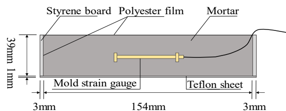
Fig. 1 Diagram of specimen for shrinkage measurement
