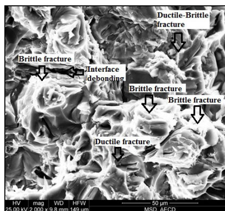
(a) Strain rate 10^{-3} s ^{-1}
