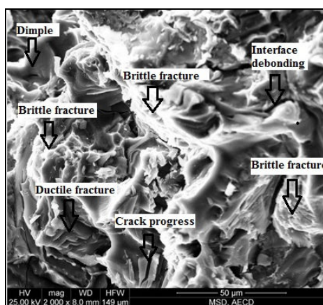
(b) Al-6Si-0.5Mg-2Ni-2Cu
