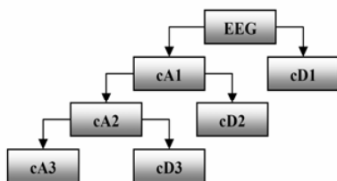
Fig. 5 Sub-band coding algorithm of the DWT
