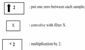
Fig. 3 The algorithm of the IDWT
