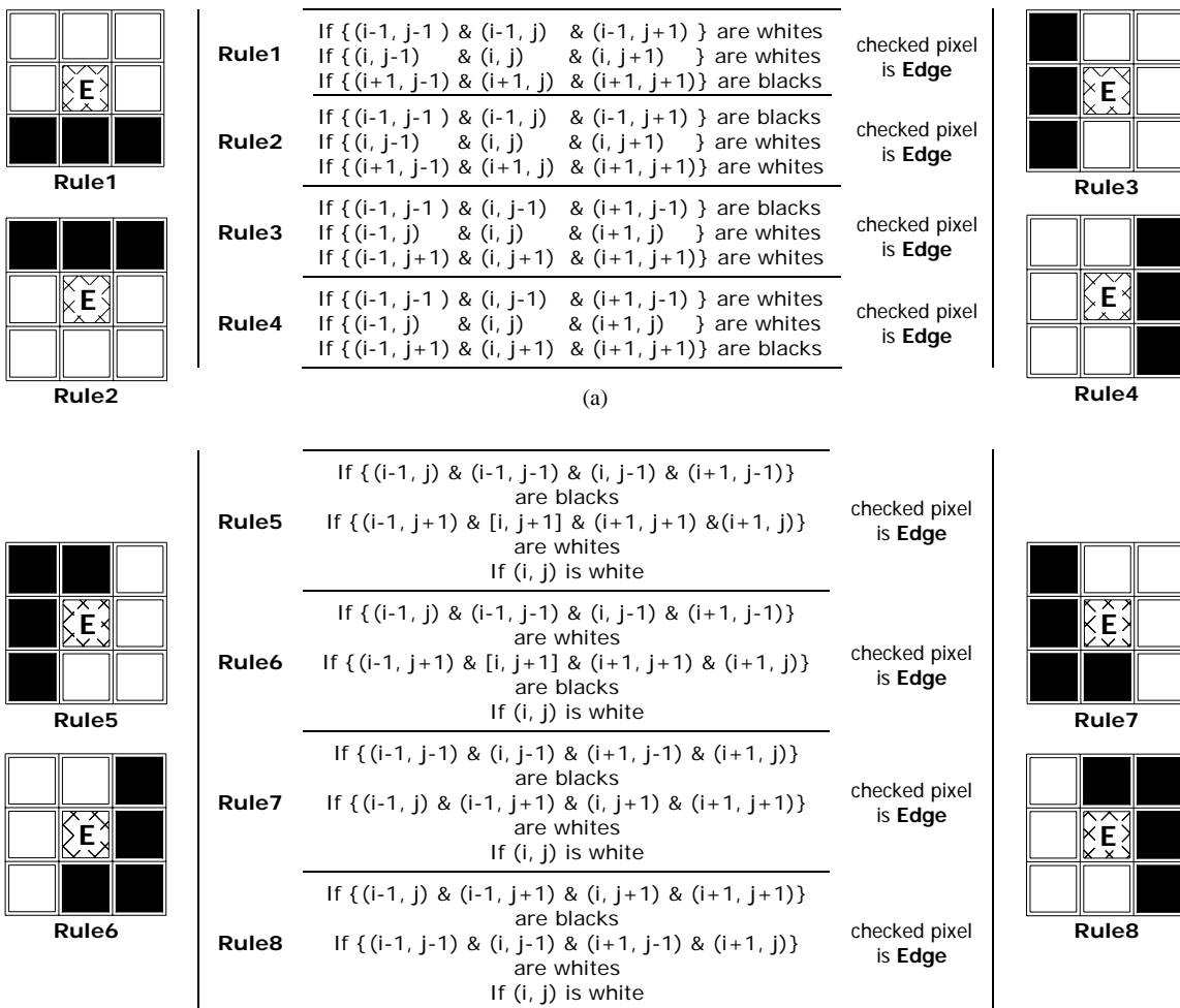
(b) Fig. 4 The Fuzzy System rules
