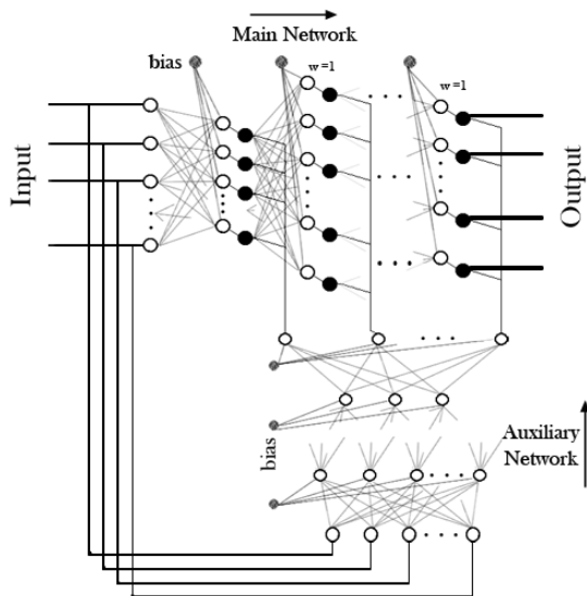
Fig 4 Overall layout of the auxiliary net model
