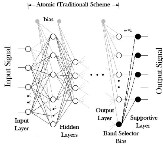
Fig 3 NN Scheme with supportive layer
