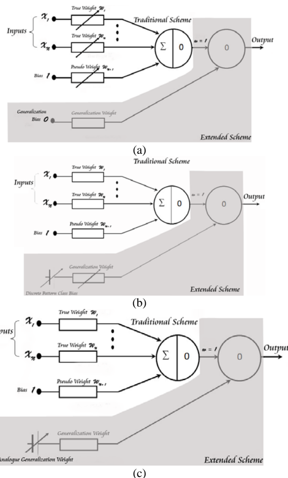
Fig 2 Perceptron adaptation modeling
