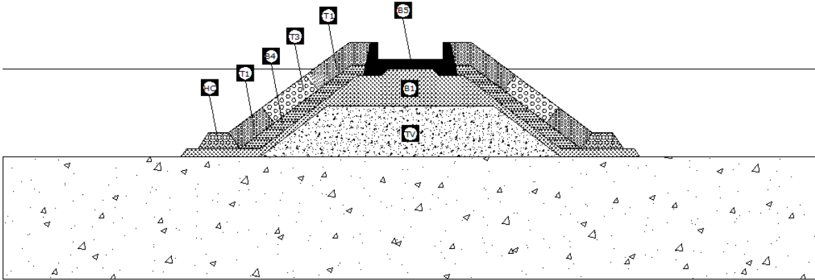
Fig. 3 The different elements constituting the dyke
