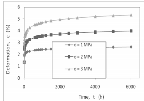
Fig. 8 Middle-time creep curves for various values of axial stress " \sigma ". (Salty medium)
