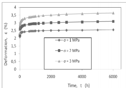
Fig. 6: Middle-time creep curves for various values of axial stress " \sigma ". (Ambient medium)
