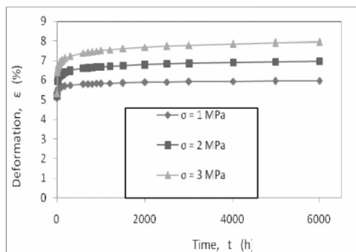
Fig. 7 Middle-time creep curves for various values of axial stress " \sigma ". (Foam medium)
