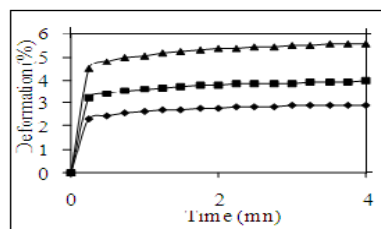
Fig. 5 Short-time creep curves for a foam middle
