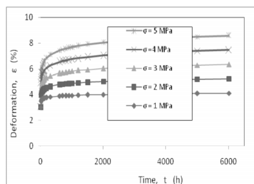
Fig. 9 Middle-time creep simulation for various values of axial stress " \sigma ". (All mediums)
