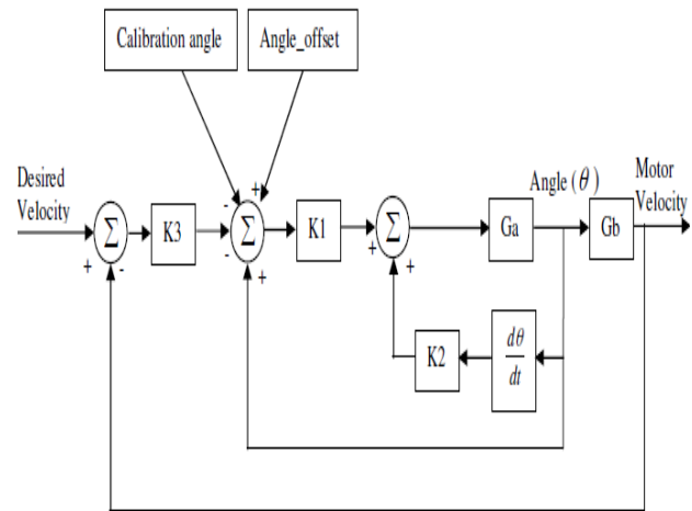
Fig. 1 Digital Cascade Control Loop for Robot
