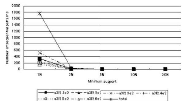
(d) Second sequential patterns (Number of items=3, Number of levels=5)
