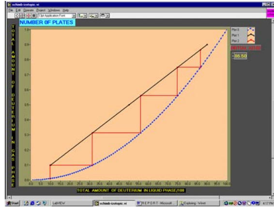
Fig. 4 Front panel in LabView for equilibrium isotherm
