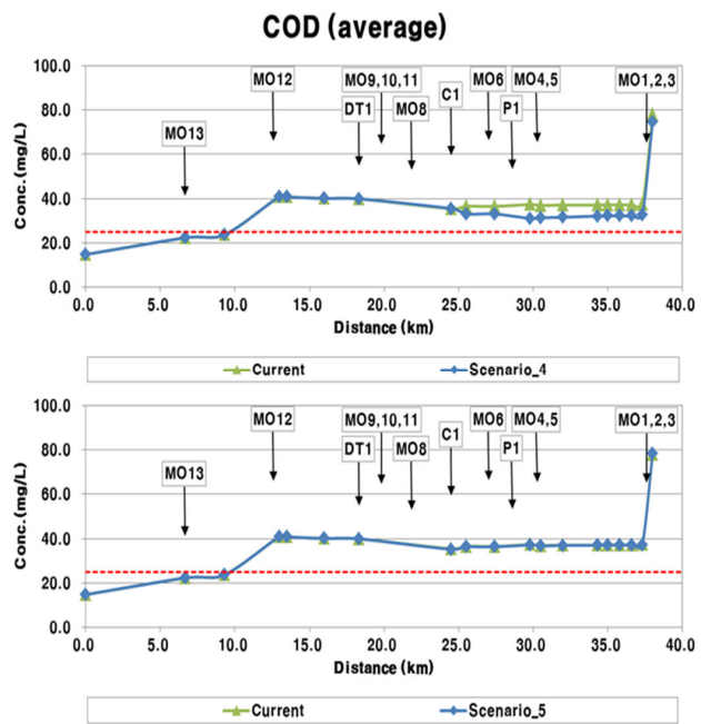
Fig. 6 Comparison of Predicted and Measured Spatial COD Concentrations for Scenario 4 and 5
