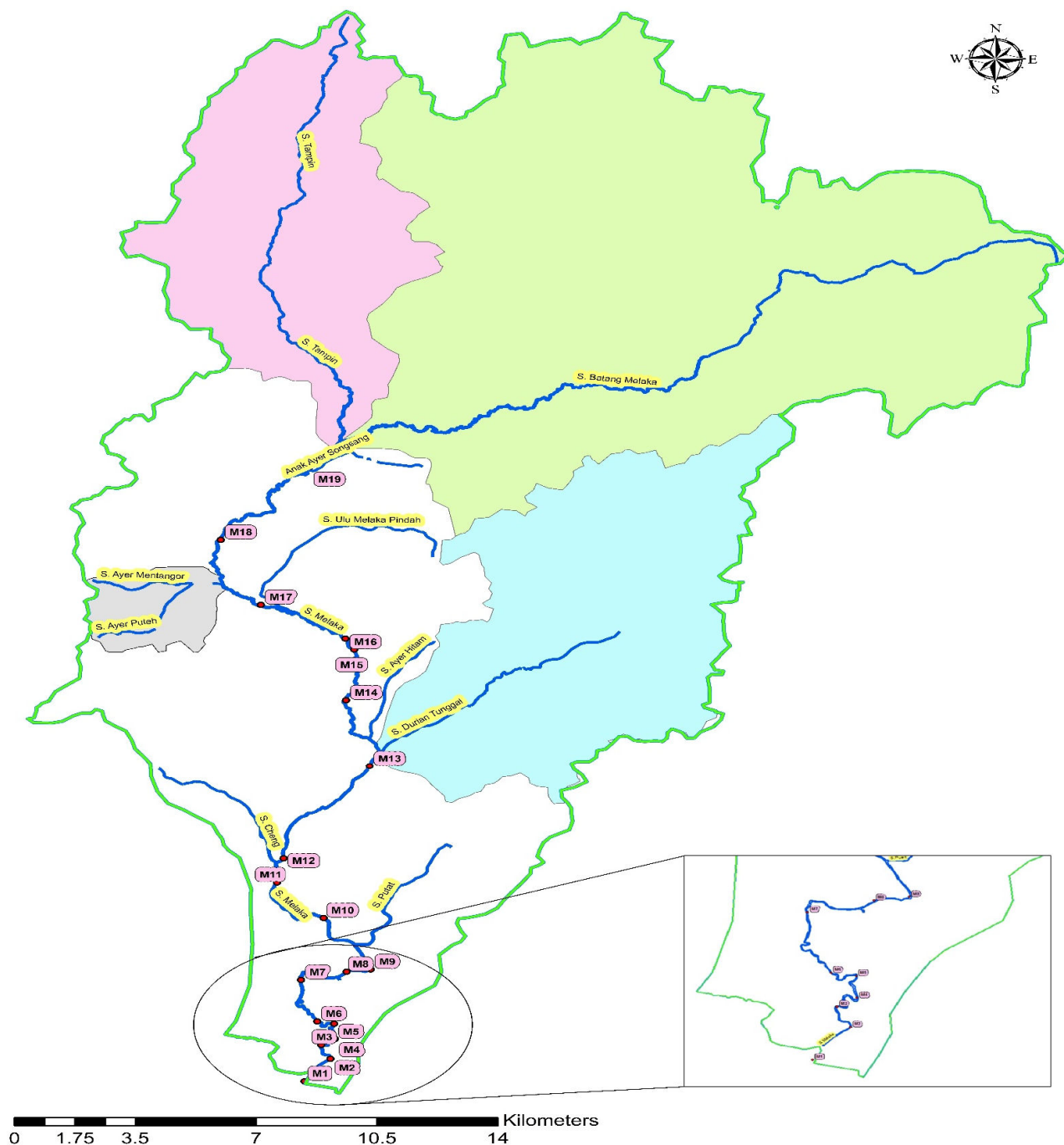
Fig. 1 Malacca River and its tributaries
