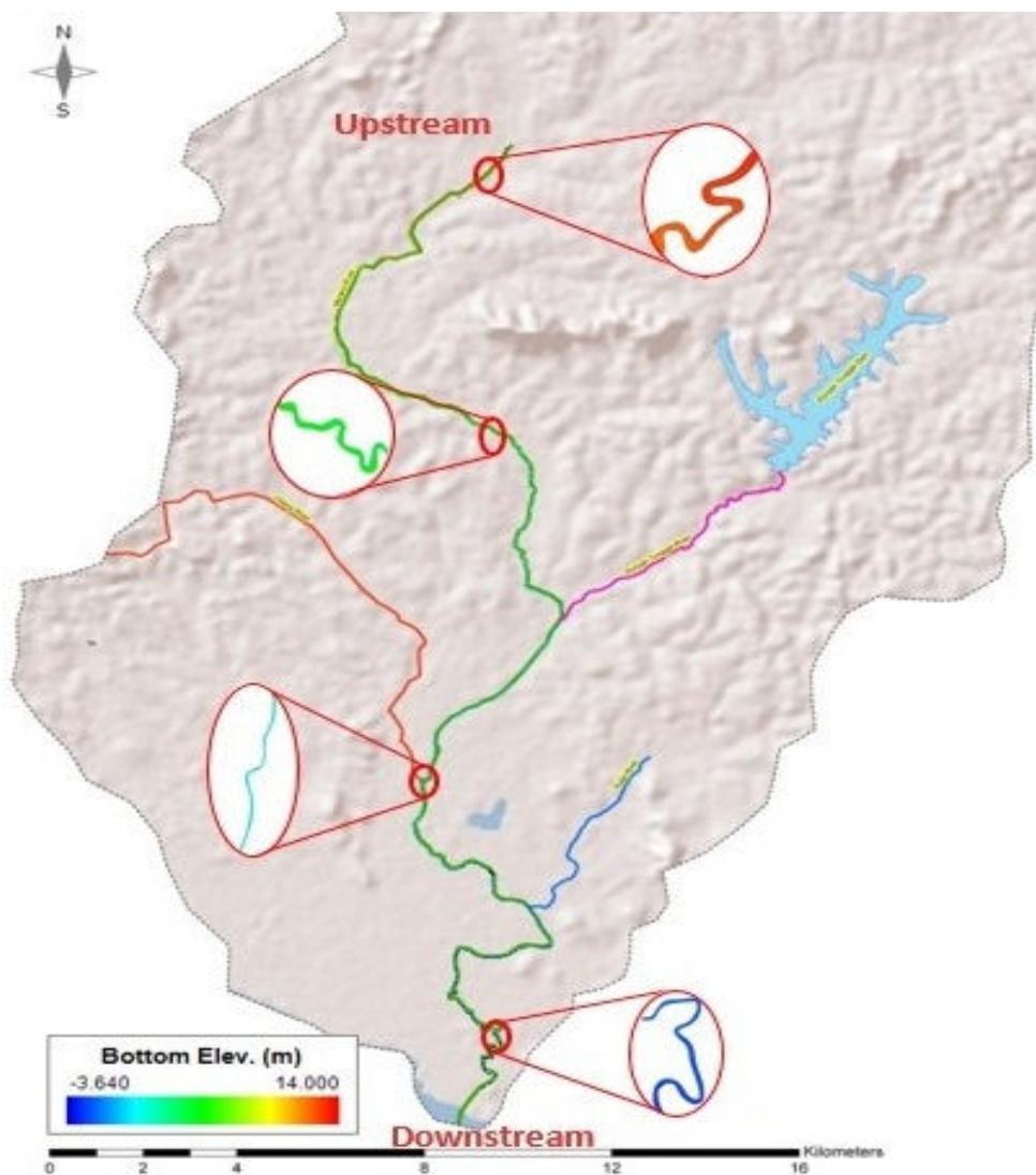
Fig. 2 Segmentation of Malacca River
