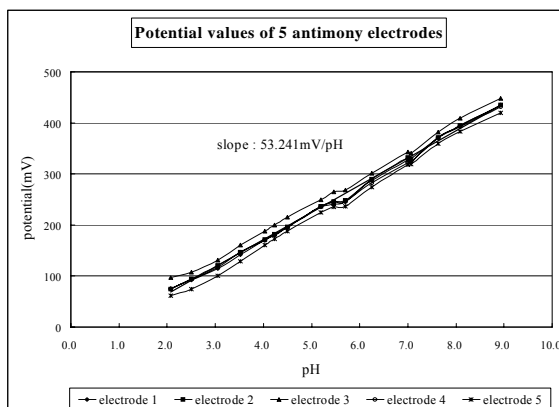
Fig. 6 Potential values of 5 antimony electrodes
