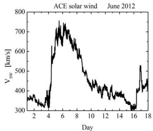
Fig. 5. Solar wind speed from ACE satellite measurements [21], for June 1-18, 2012.
