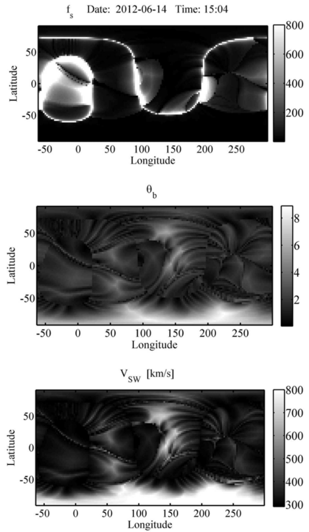
Fig. 4. (a) Magnetic flux tube expansion factor f_s , (b) nearest coronal hole boundary factor \theta_b , and (c) solar wind speed V_{sw} at R_s . The synoptic magnetogram used as the input for the code is from June 14, 2012 (15:04UT).
