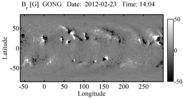
Fig. 1. Observed photospheric radial component of the magnetic field B_r(R_0, \theta, \phi) from the GONG synoptic magnetogram. The longitude 0^\circ corresponds to the central meridian on February 23, 2012 (14:04UT). The left side from the central meridian is towards the east of the Sun. The magnetic field scale is saturated at \pm 50\text{G} .
