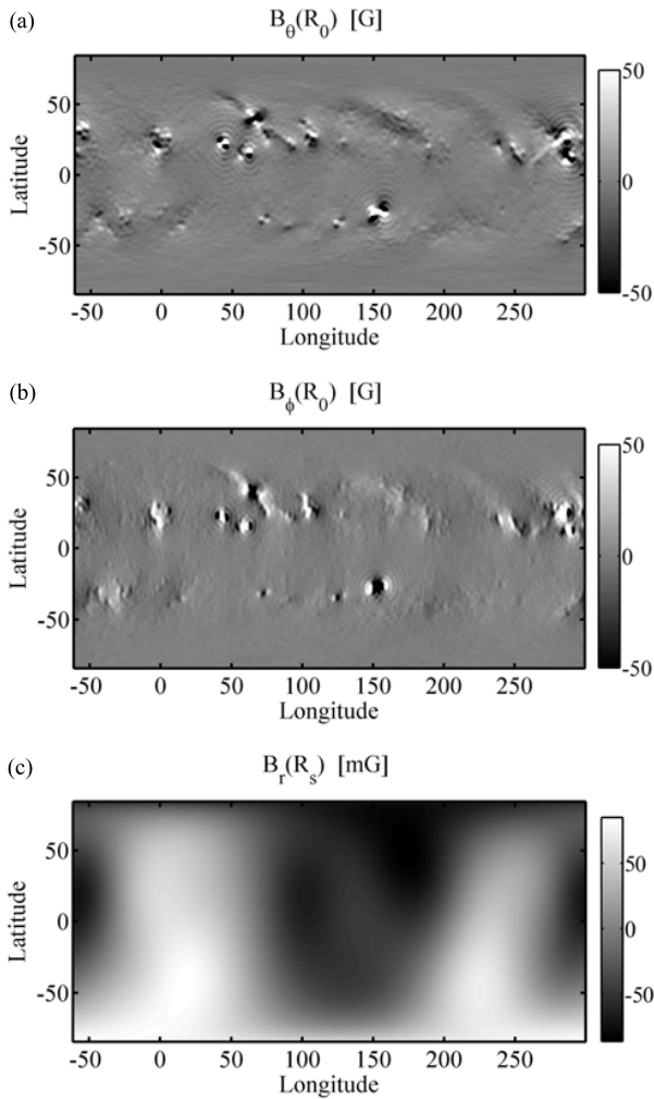
Fig. 3. Solution for the photospheric magnetic field components (a) B_\theta and (b) B_\phi with n_{max} = 120 . The magnetic field scale is saturated at \pm 50 G. (c) Solution for the radial component of the magnetic field B_r at source surface R_s with n_{max} = 120 .
