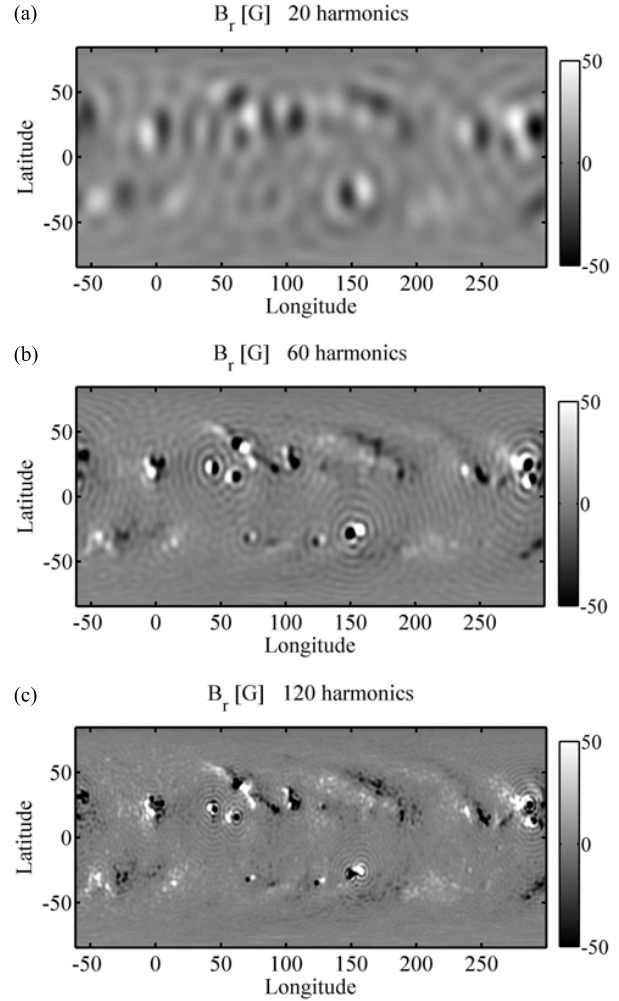
Fig. 2. Photospheric radial component of the magnetic field B_r(R_0, \theta, \phi) calculated with (a) n_{max} = 20 , (b) n_{max} = 60 , and (c) n_{max} = 120 . The magnetic field scale is saturated at \pm 50\text{G} .
