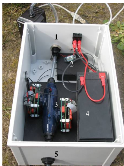
Fig. 3 Internal layout of System I
