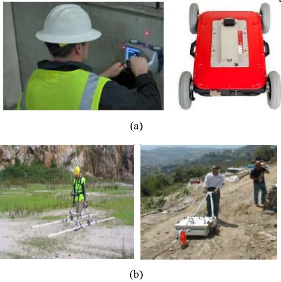
Fig. 2 (a) Commercial StructureScan and GroundExplorer GPR; (b) GPR scanning of archaeological site using low frequency 100 MHz GPR systems
