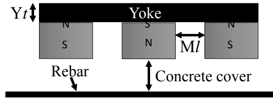
Fig. 8 Proposed structure of the adhesion module
