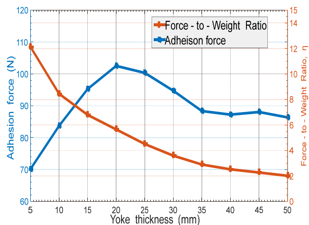
Fig. 10 Adhesion force and Force-to-Weight Ratio for different thicknesses of the yoke, Y_t [18]
