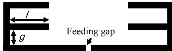
Fig. 6 Proposed miniature 200 MHz dipole antenna
