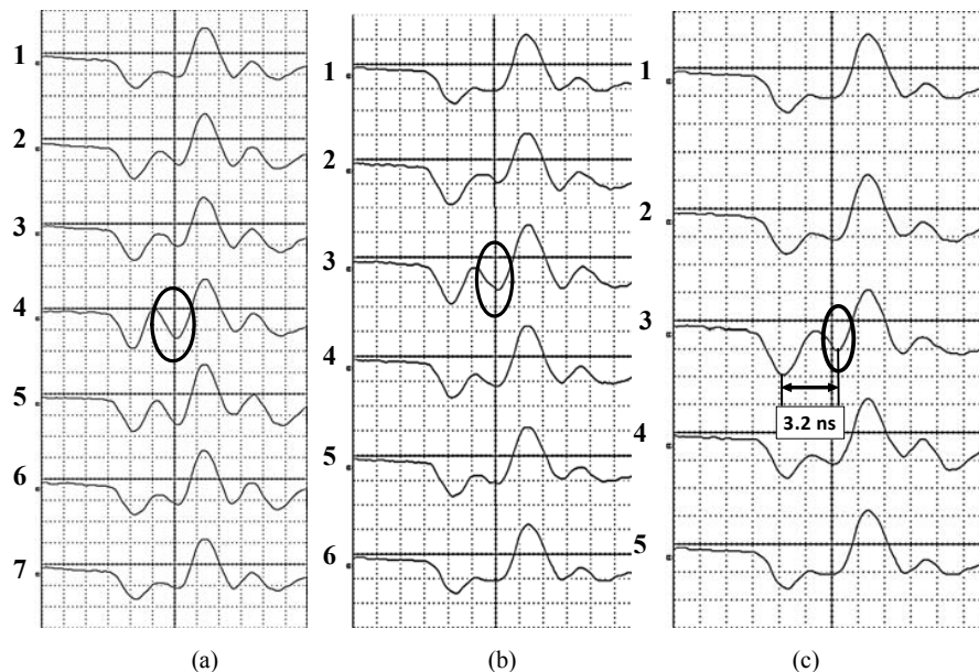
Fig. 15 Peak of the reflection from the target objects (shown in circle) for: (a) aluminium sheet; (b) aluminium block; (c) rebar.
