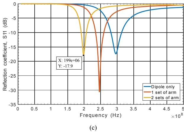
Fig. 7 Reflection coefficient, S11 values for: (a) different lengths extra of radiating arm, l ; (b) different gap between the arms, g ; (c) number of extra radiating arm sets
