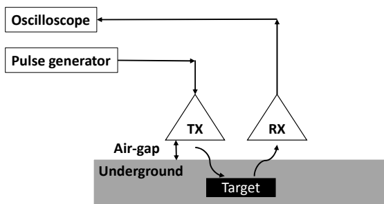
Fig. 5 Block diagram of the GPR
