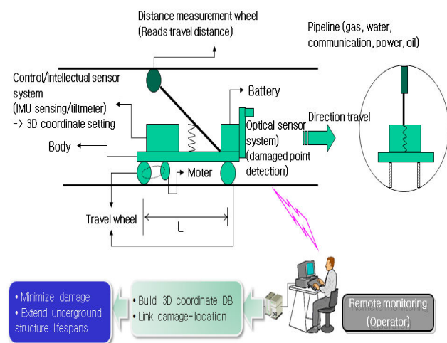
Fig. 2 Schematic Diagram of the System
