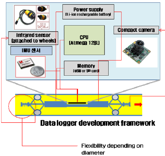
Fig. 3 Data Logger Diagram Containing IMU Sensor
