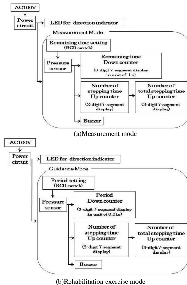
Fig. 6 Structure of electrical circuit
