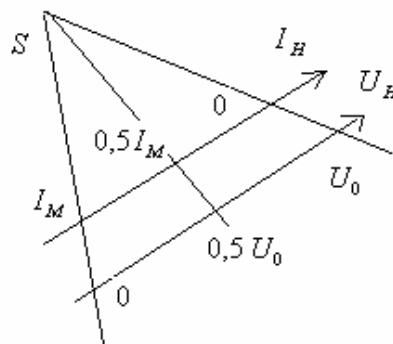
Fig. 5 Affine transformation
