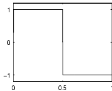
Fig. 3 Characteristic of mother wavelet Haar
