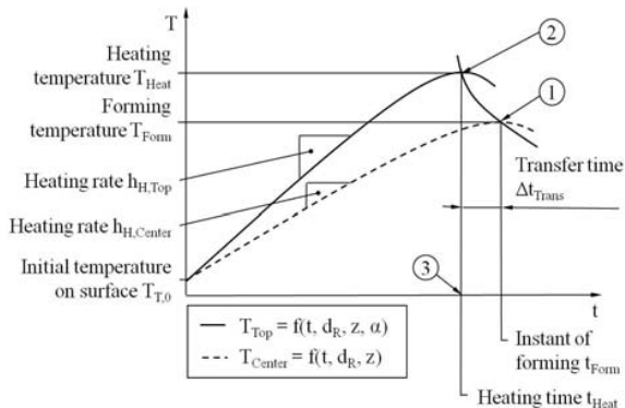
Fig. 17 Procedure for the determination of process parameters for composite heating
