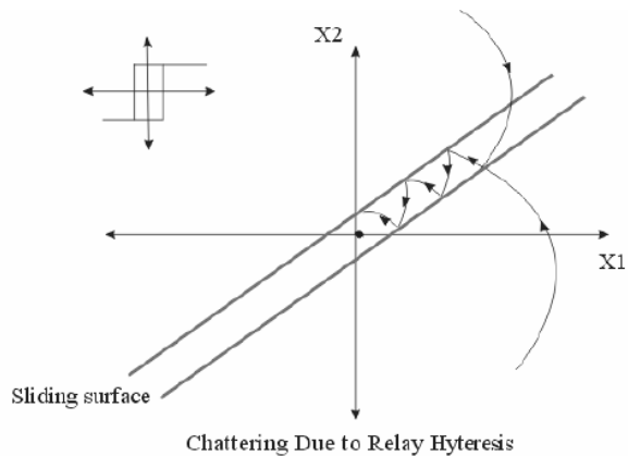
Chattering Due to Relay Hysteresis Fig. 6 Chattering phenomenon.
