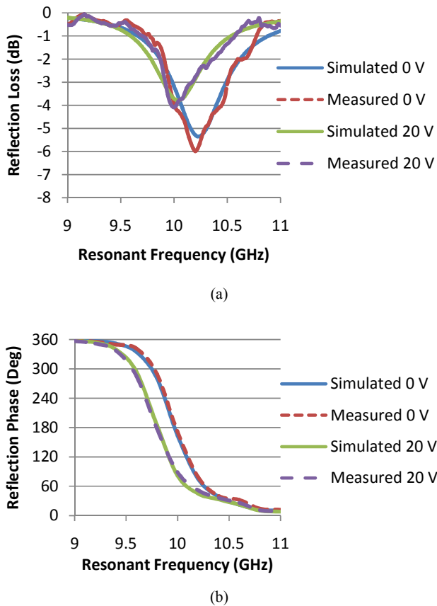
Fig. 8 Comparison of measured and simulated results for circular slot embedded patch element (a) reflection loss curve and (b) reflection phase curve
