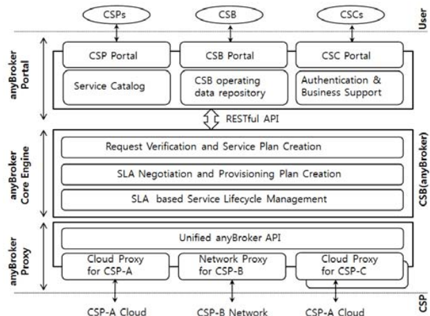
Fig. 1 anyBroker whole architecture
